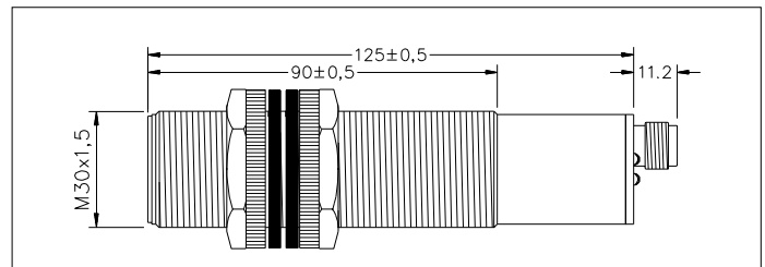
Dimensions/Abmessungen/Dimensions
